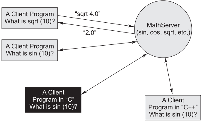
Fig. 13.6 A socket-based math server and clients
