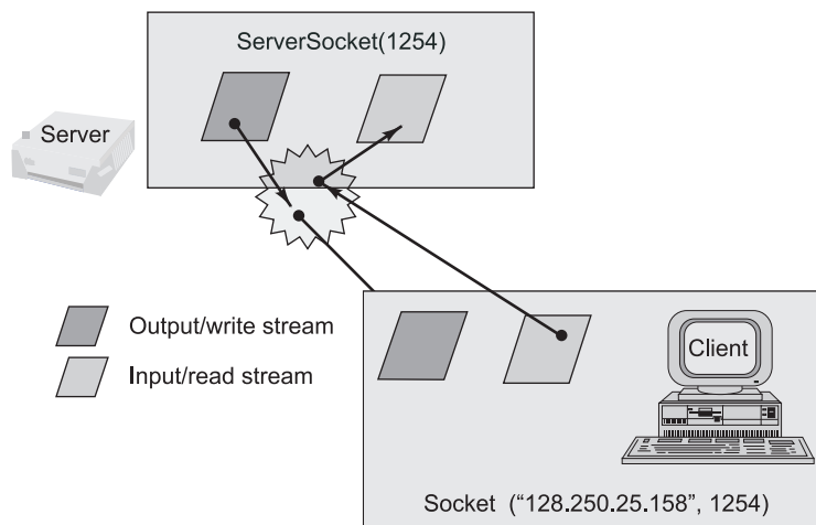
Fig. 13.5 Socket-based client and server programming
