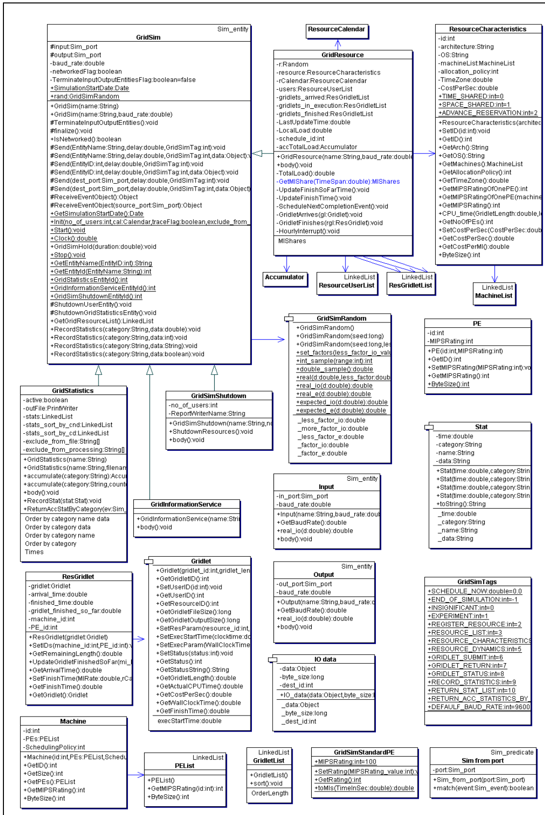
Figure 4: Class diagram of gridsim package.
