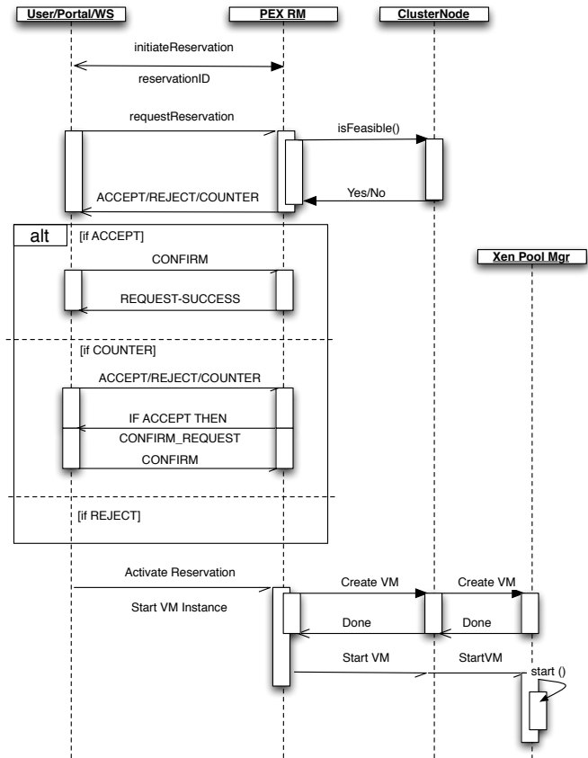
Figure 2. Alternate Offers Negotiation for Advance Reservations.
