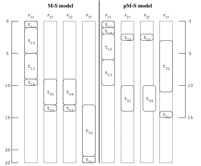
Figure 4. Comparison of the finish time of subtasks in Figure 2 under M-S model and pM-S model.
