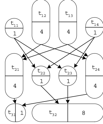
Figure 2. An example task graph.
