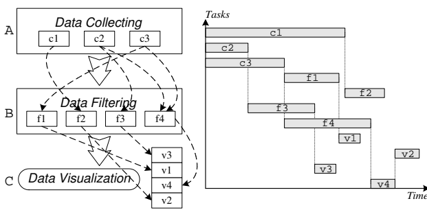
Figure 1. Optimizing the example parameter-sweep workflow.
