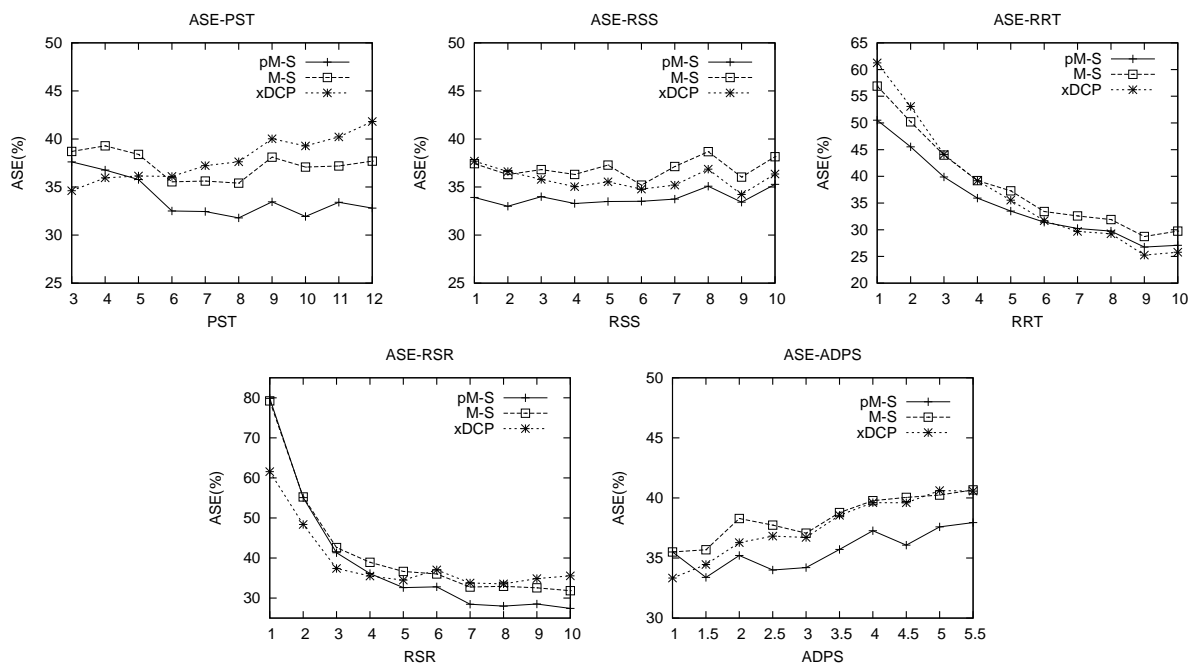
Figure 5. Average Scheduling Effectiveness (ASE) varies with PST, RSS, RRT, RSR and ADPS.
