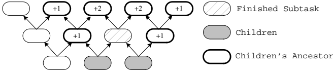
Figure 3. An example of priority calculation.
