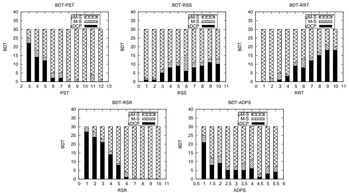
Figure 6. Average Beat-down Time (BDT) varies with PST, RSS, RRT, RSR and ADPS.
